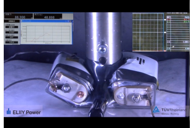
Crushing Test
